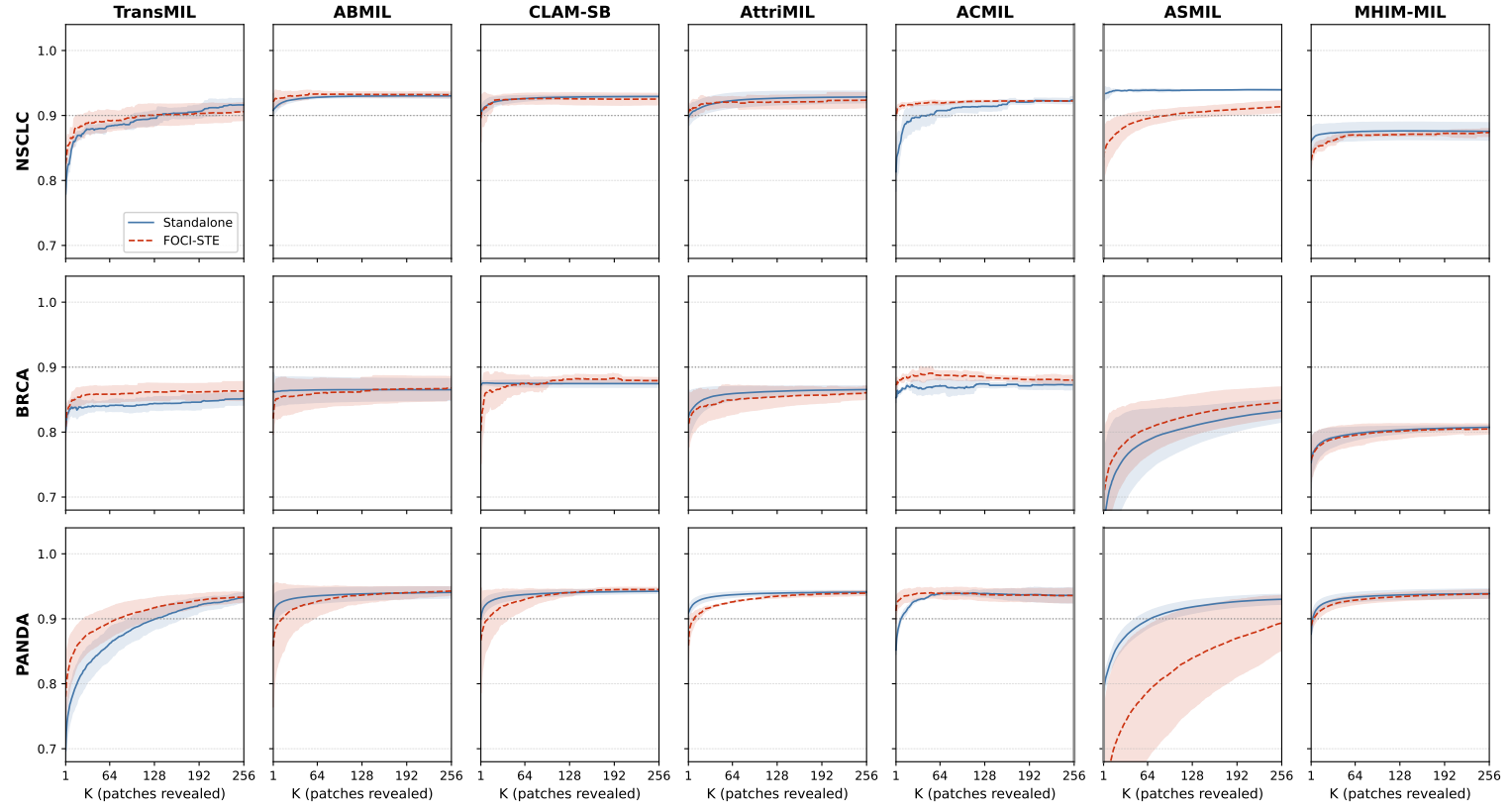
Figure 5: Extended SRP reveal curves for seven backbones \pm FOCI across NSCLC, BRCA, and PANDA. Curves show the full confidence- K trajectories behind Tables 12–14; blue solid = standalone backbone, red dashed = FOCI-augmented, shaded = \pm 1 std over three seeds, dotted line = \kappa = 0.9 .
