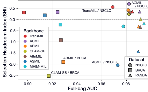
Figure 3: Slide-level AUC and SHI are decoupled. Each point is a (backbone, dataset) pair; color denotes backbone and marker shape denotes dataset. High-AUC backbones can have near-zero or negative SHI when their native ranking saturates or conflicts with an external readout, while TransMIL and ACMIL maintain positive SHI without necessarily being the best full-bag classifiers.
